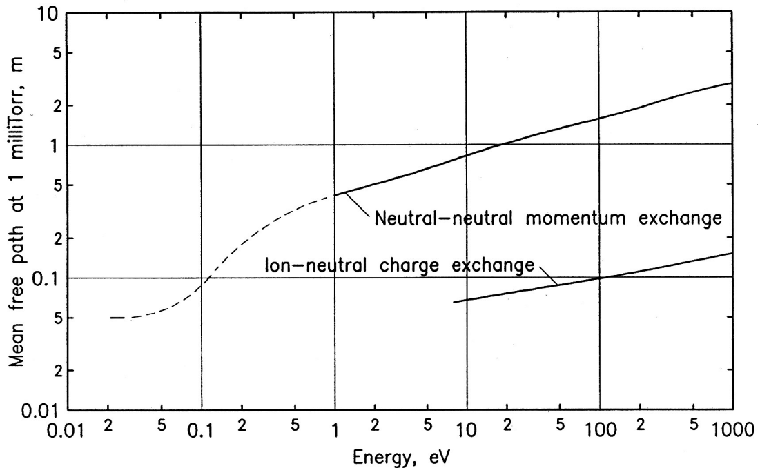
Fig. 1. Charge-exchange and momentum-exchange path lengths for argon.
